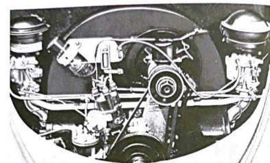
The US-made Diets manifold employs stock VW carburetors with the factory setting. Note bracket plate for the dual throttle linkage.
